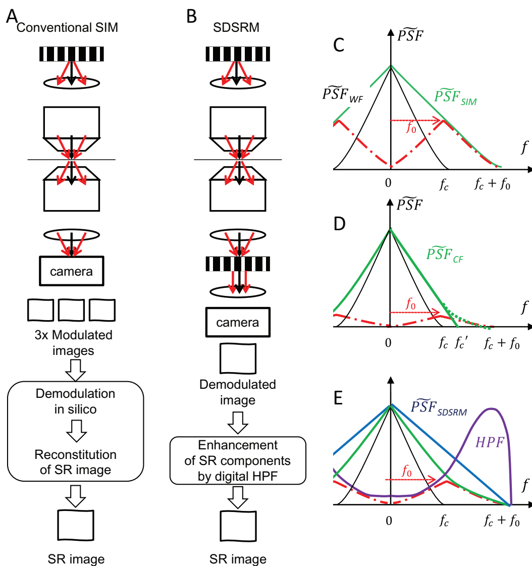
FIGURE 1: Principles of SIM and SDSRM. (A, B) Schematic comparison of SIM and SDSRM. (C) Fourier transform of the point spread function (PSF) of SIM, \widehat{PSF}_{SIM} (green), is a weighted sum of \widehat{PSF}_{WF} (black) and its frequency ( f_0 )-shifted SR components (red). Here f_c denotes the cut-off frequency of conventional WF, and f_0 denotes the spatial frequency of the SIM illumination pattern. (D) Fourier transform of the PSF of CF, \widehat{PSF}_{CF} (green), is a weighted sum of \widehat{PSF}_{WF} (black) and its frequency ( f_0 )-shifted components (red). Here f_0 denotes the basic spatial frequency of the mask pattern, and f'_c denotes the apparent cut-off frequency of CF. (E) With SDSRM, the stripe pattern is designed to increase the SR component (red), and the digital high-pass filter (purple) further enhances the SR component (blue). See Supplemental Figures S1 and S2 for details.
